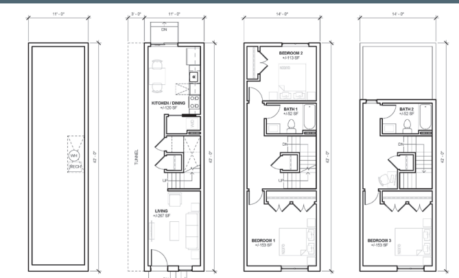
moto.designshop 062724 3-STORY + FULL TUNNEL 08 31'0" x 10'
