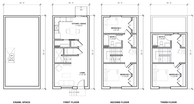
moto.designshop 062724 3-STORY WIDE 06 31'0" x 10'
