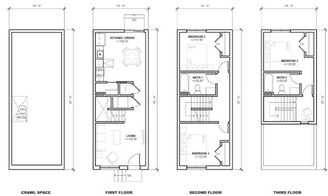
moto.designshop 062724 3-STORY WITH SETBACK 01 31'0" x 10'
