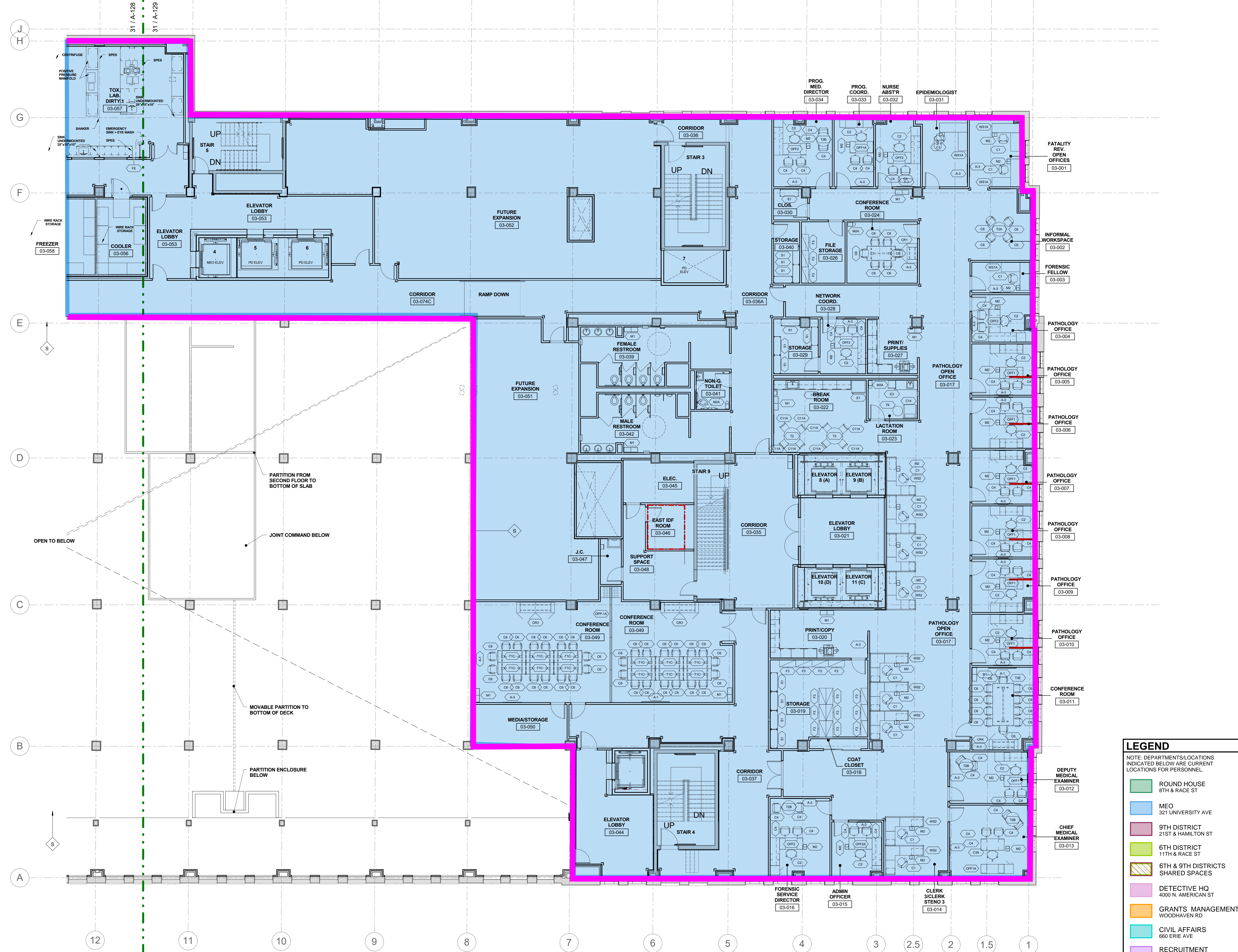
1 3RD FLOOR FURNITURE PLAN - EAST 1/8" = 1'-0"
