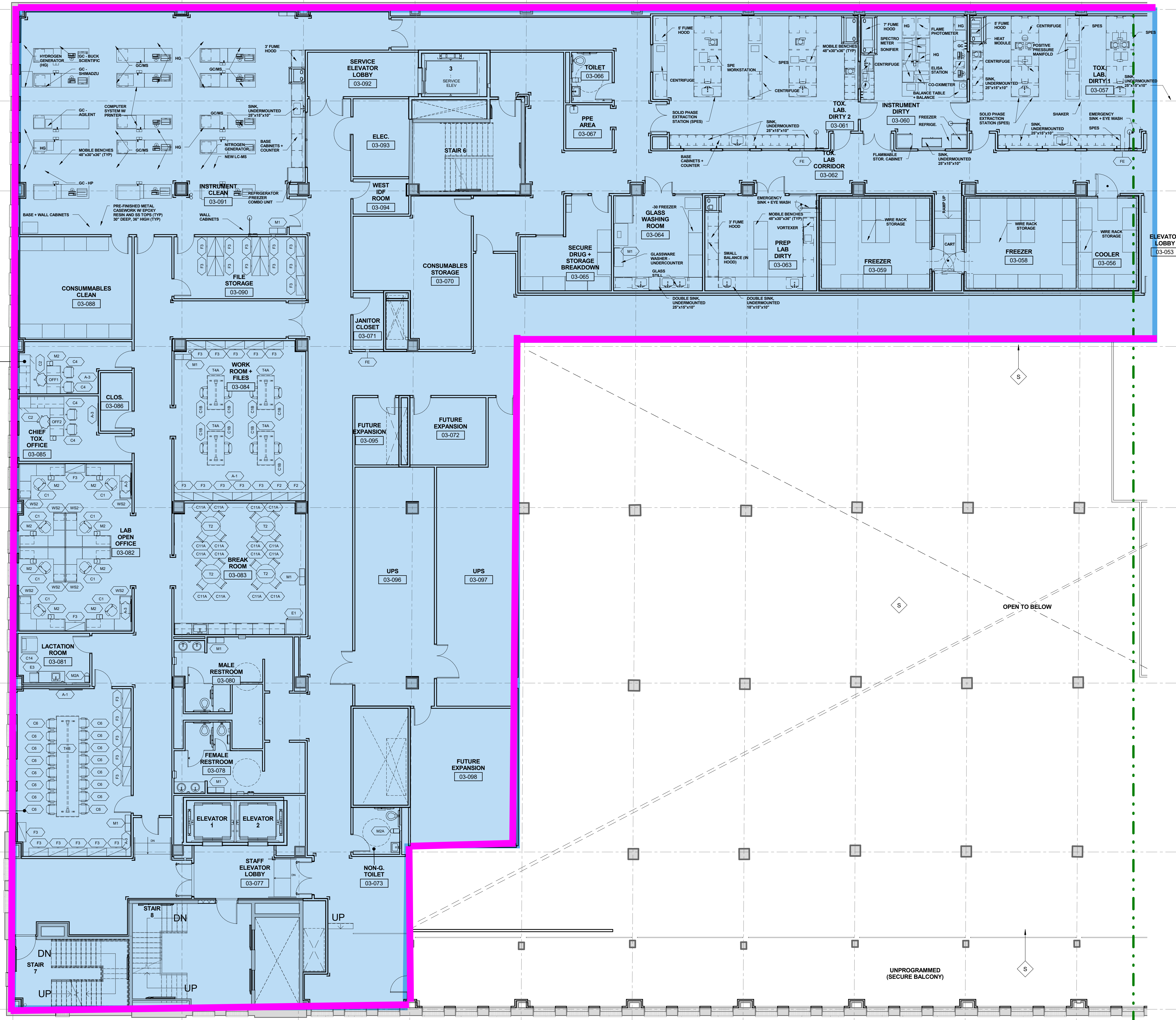
1 3RD FLOOR FURNITURE PLAN - WEST 1/8" = 1'-0"
