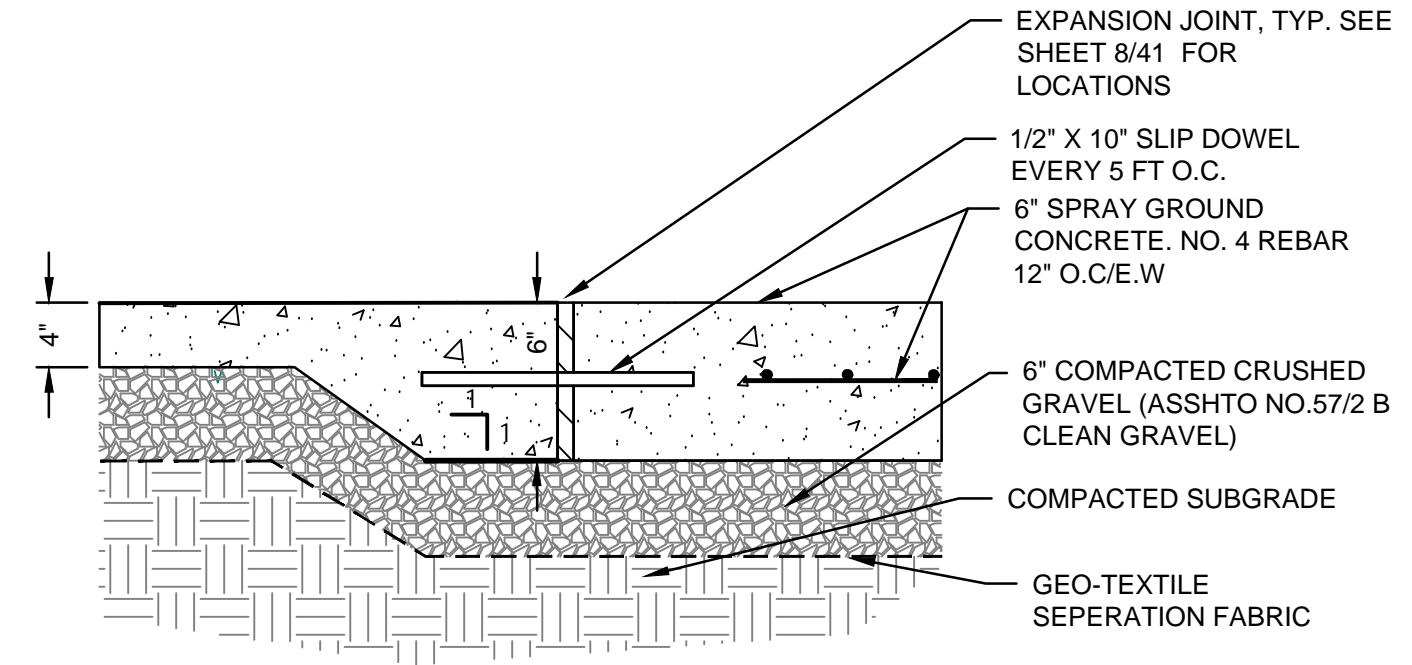
3 4" TO 6" CONCRETE DETAIL SCALE: NTS
